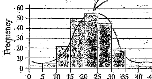
(b) Bell-shaped (symmetric)
