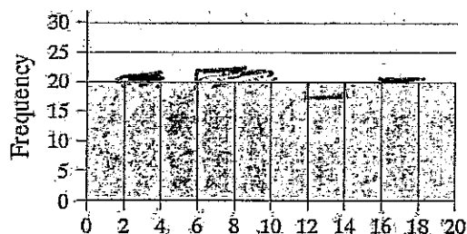
(a) Uniform (symmetric)
