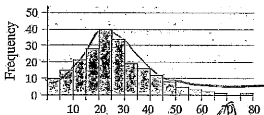
(c) Skewed Right
